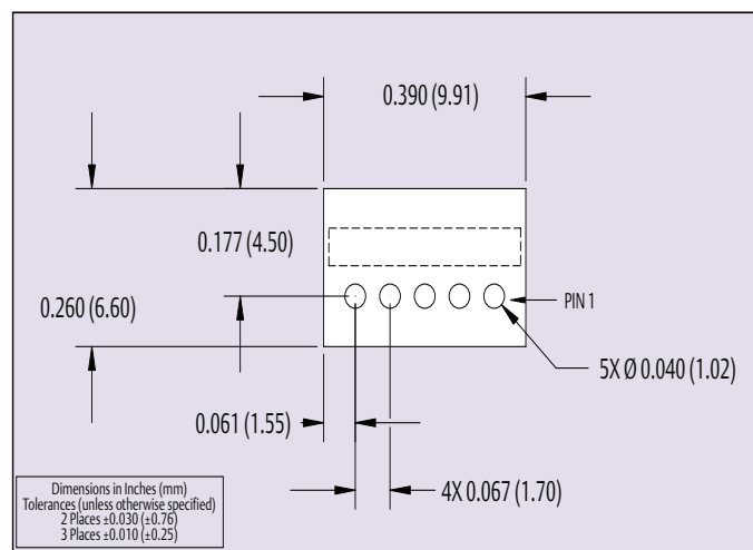
Figure 4C - LDO06C/10C SMT Recommended Footprint
