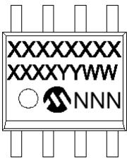
8-Lead SOIC (150 mil) (MCP6546, MCP6547, MCP6548, MCP6549)
