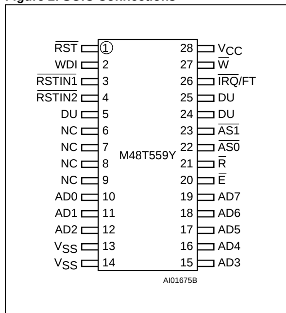
Figure 2. SOIC Connections
