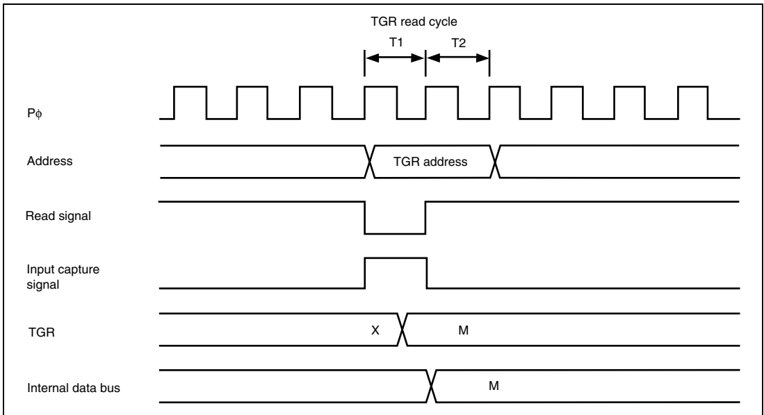
Figure 10.76 Contention between TGR Read and Input Capture
