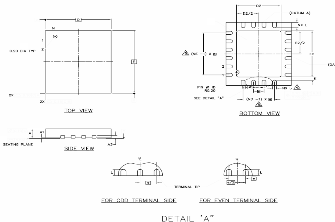
Figure 103. QFN 5x6: 20-Lead Very Thin Fine Pitch Quad Flat No-Lead Package
