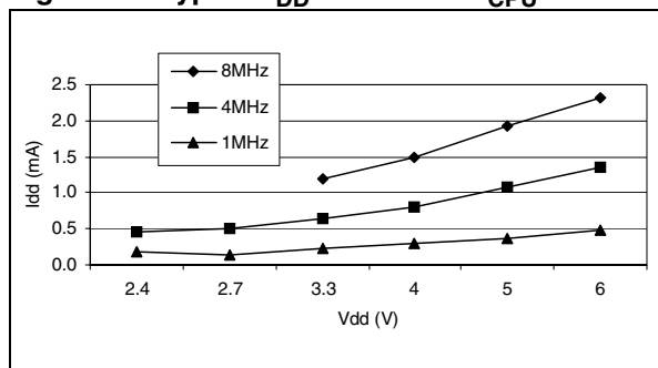
Figure 77. Typical I_{DD} in WAIT vs f_{CPU}
