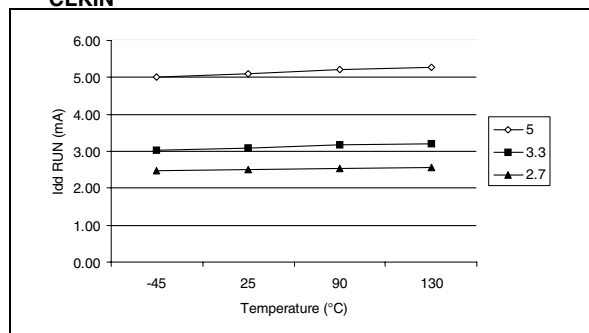
Figure 80. Typical I_{DD} vs Temperature and V_{DD} at f_{CLKIN} = 16\text{ MHz}
