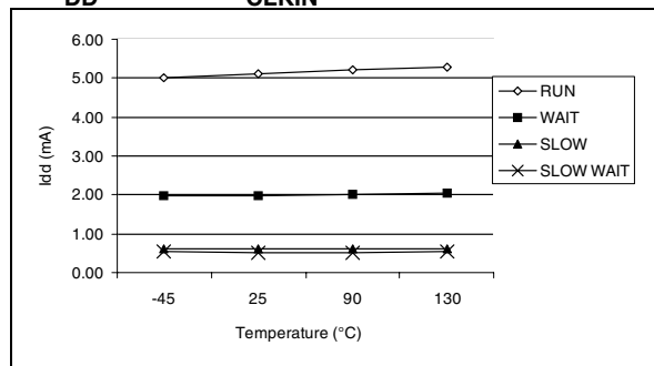
Figure 80. Typical I_{DD} vs Temperature and V_{DD} at f_{CLKIN} = 16\text{ MHz}
