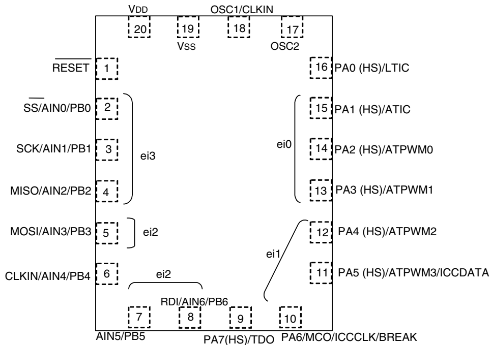
Figure 3. 20-Pin QFN Package Pinout
