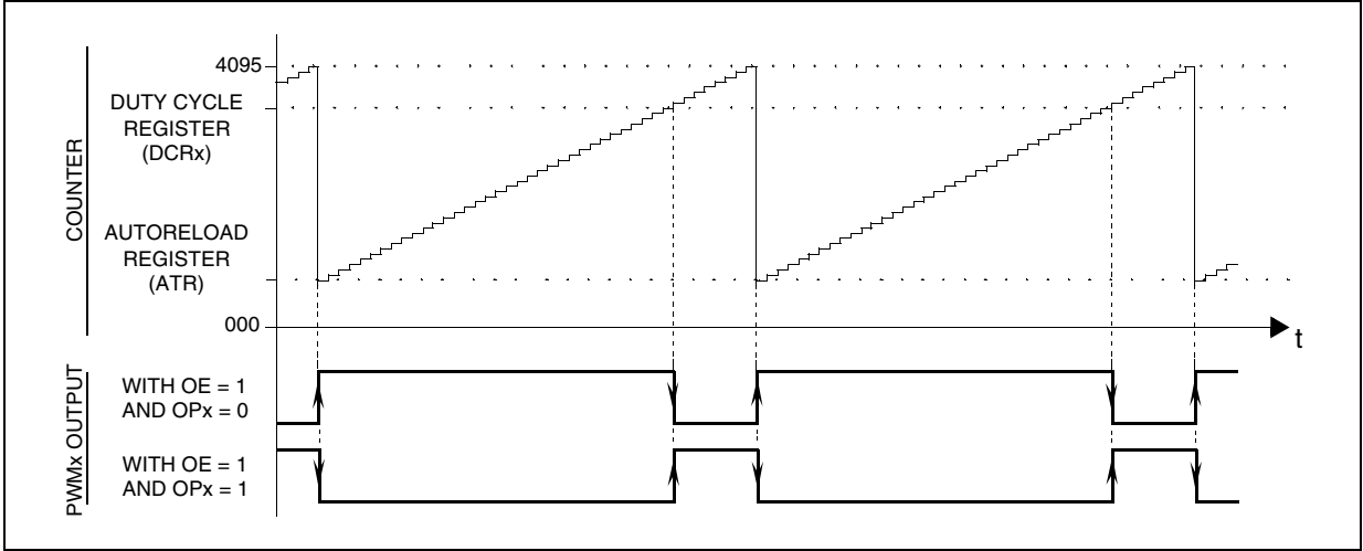
Figure 37. PWM Function
