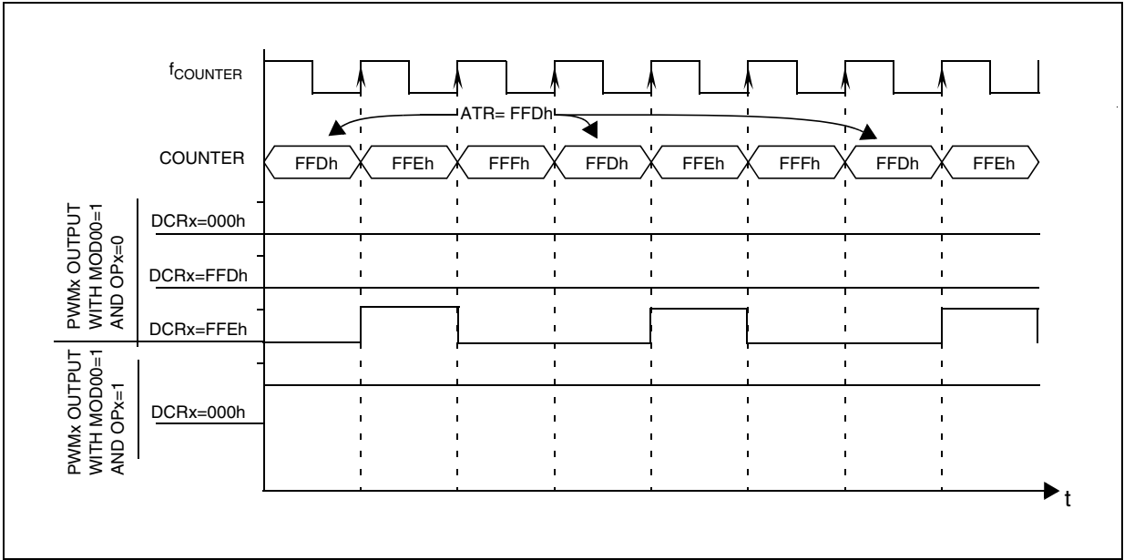
Figure 38. PWM Signal from 0% to 100% Duty Cycle
