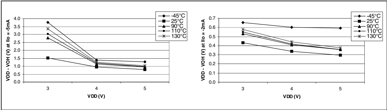
Figure 94. Typical V_{DD} - V_{OH} vs V_{DD}
