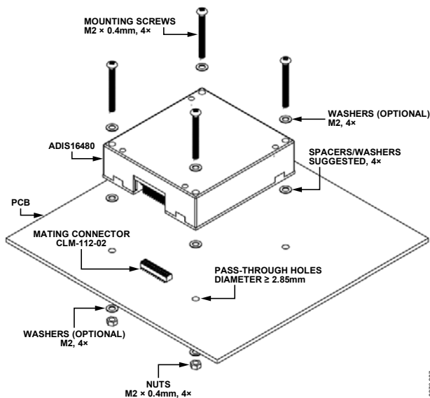
Figure 27. Mounting Example
