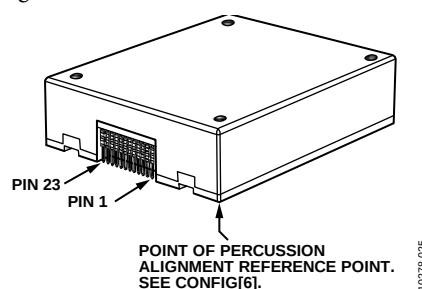
Figure 25. Point of Percussion Reference Point
