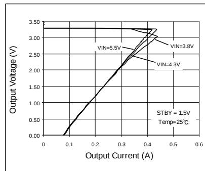
Fig. 157 OCP Threshold
