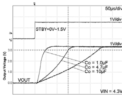
Fig. 174 Start Up Time I_{out} = 200\text{mA}
