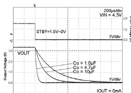
Fig. 177 Discharge Time I_{out} = 0\text{mA}
