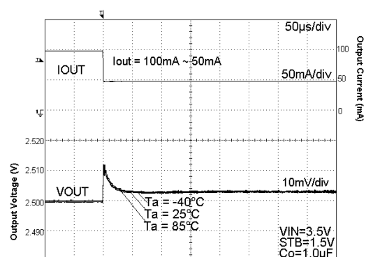
Fig. 81 Load Response
