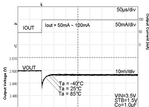
Fig. 80 Load Response
