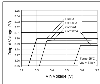
Fig. 151 Line Regulation
