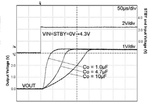
Fig. 175 Start Up Time (STBY=VIN) I_{out} = 0\text{mA}
