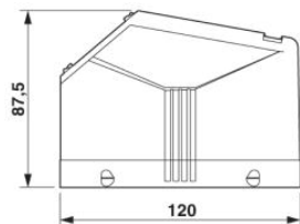
Dimensioned drawing
