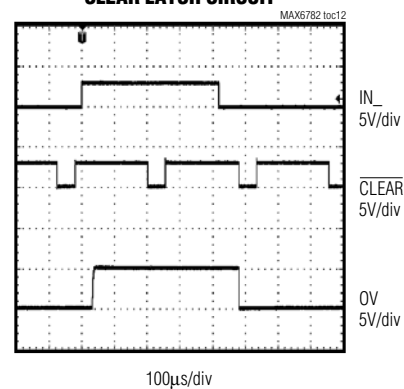
CLEAR LATCH CIRCUIT
