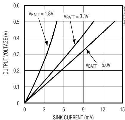
\overline{LBO} OUTPUT VOLTAGE LOW vs. SINK CURRENT
