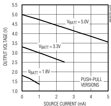
\overline{LBO} OUTPUT VOLTAGE HIGH vs. SOURCE CURRENT
