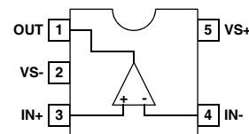
EL5192 (5 LD SOT-23) TOP VIEW
