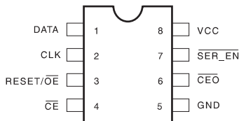
8-Pin DIP
