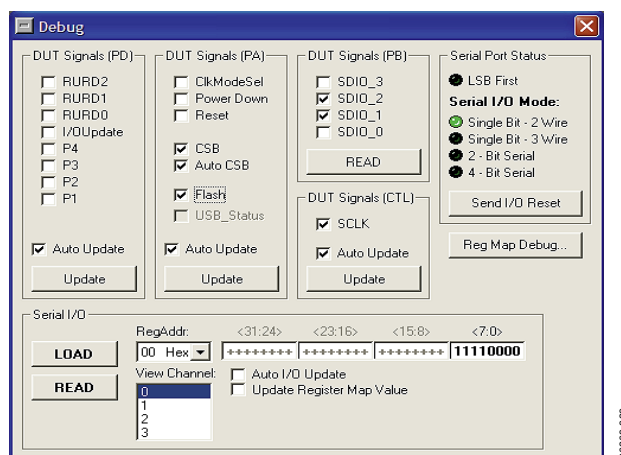
Figure 20. Debug Window
