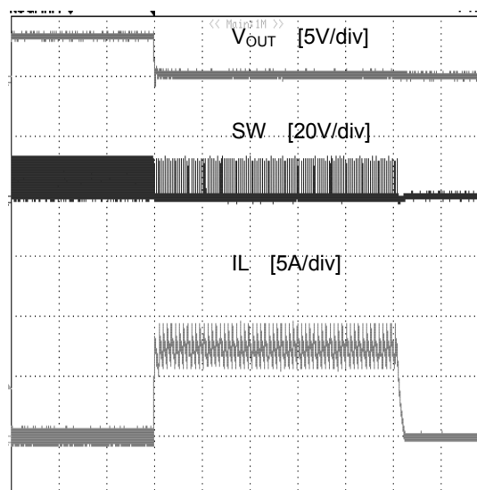
Figure 15. OCP Function ( V_{IN}=12V , V_{OUT}=3.3V , L=4.7\mu H , C_{out}=44\mu F , V_{OUT} is short to GND)
