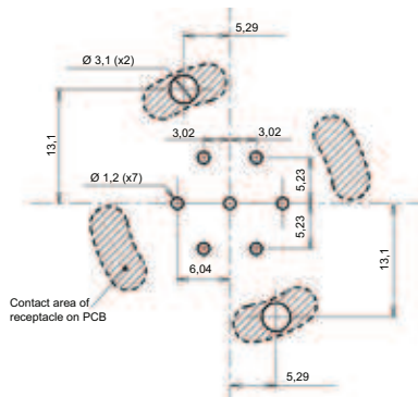
DRILLING PATTERNS
