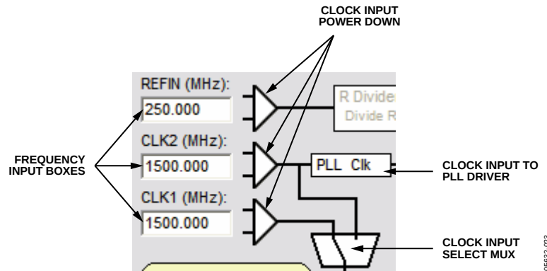
Figure 23. Clock Inputs, Main Interface Window
