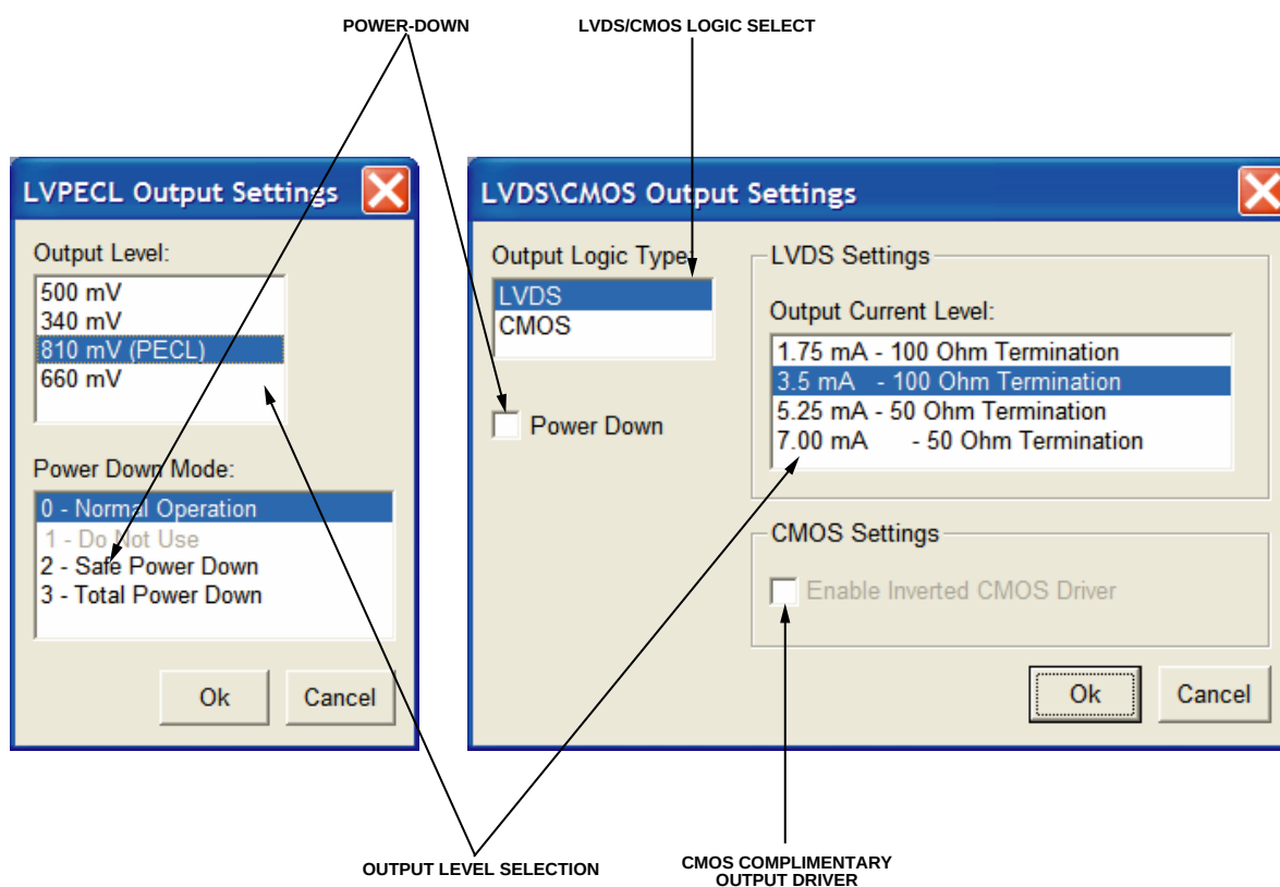
Figure 27. Output Settings Windows
