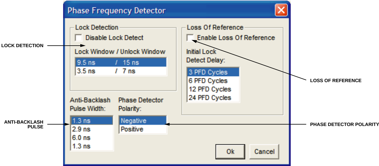
Figure 19. Phase Frequency Detector Window
