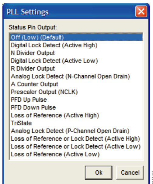
Figure 22. PLL Settings Window
