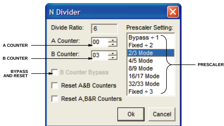
Figure 18. N Divider Window
