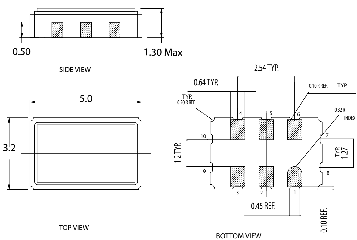
Figure 8. 6-Pin 3.2 × 5.0 mm Ceramic LCC LZ06A
