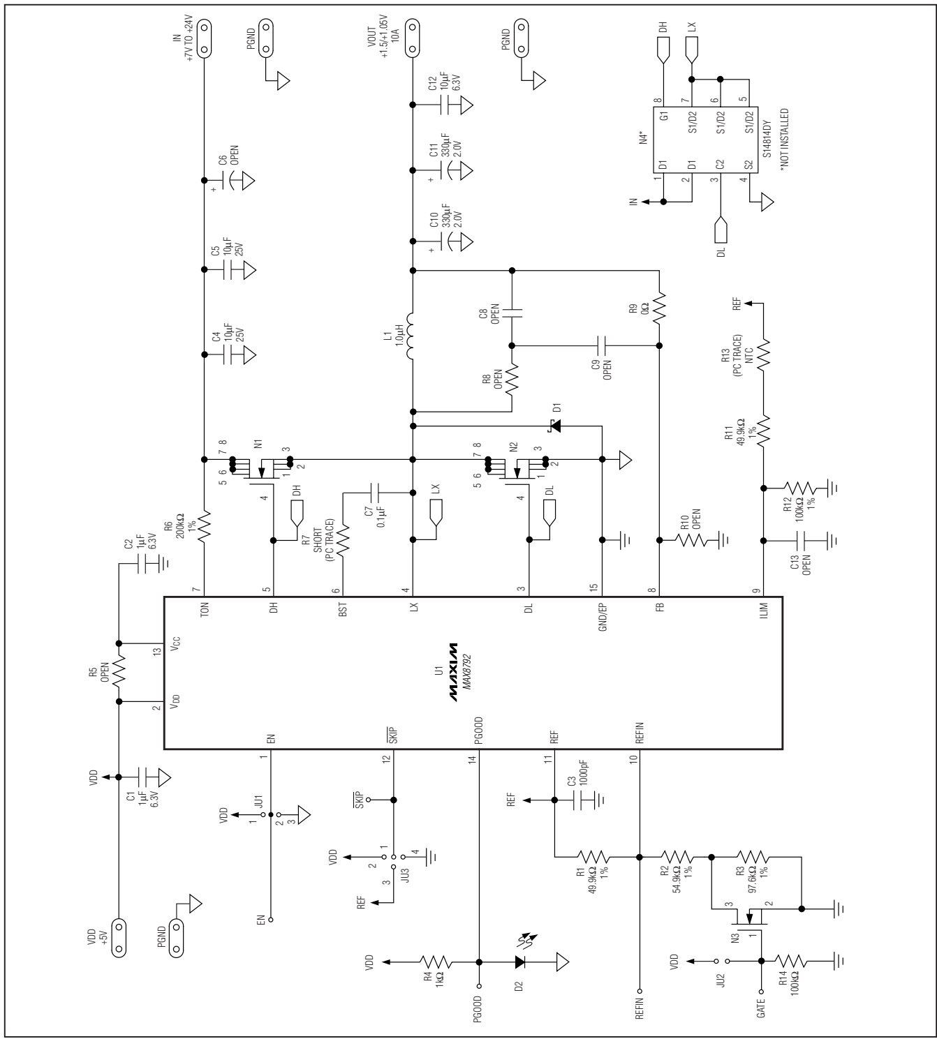
Figure 1. MAX8792 EV Kit Schematic
