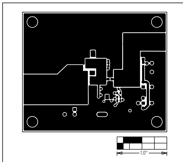
Figure 3. MAX8792 EV Kit PCB Layout—Component Side
