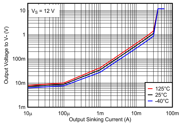
Figure 4-4. Output Voltage vs. Output Sinking Current, 12V
