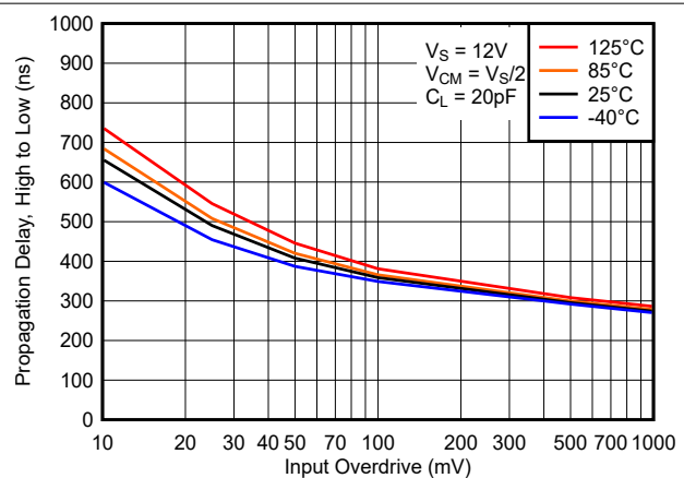
Figure 4-6. Propagation Delay, High to Low, 12V
