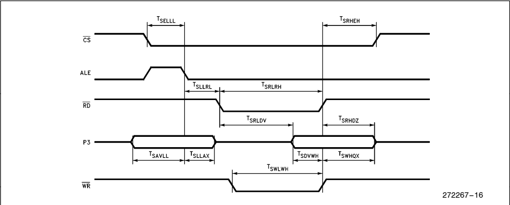
SLAVE PORT WAVEFORM—(SLPL = 1)
