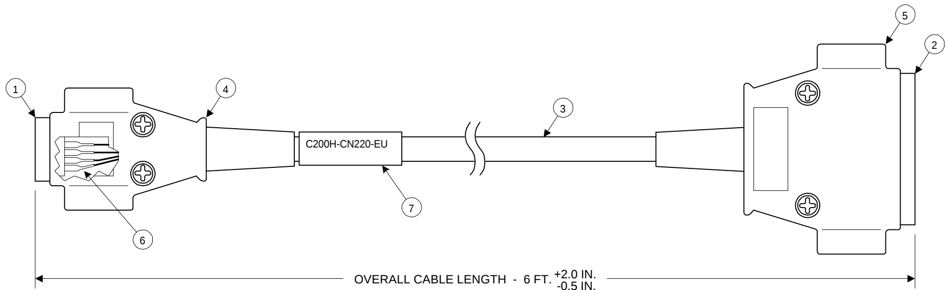
CABLE C200H-CN220-EU
