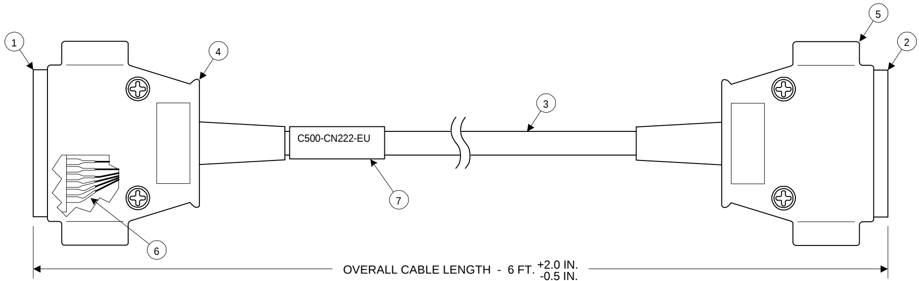
CABLE C500-CN222-EU
