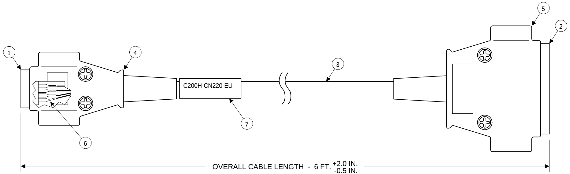
CABLE C200H-CN220-EU
