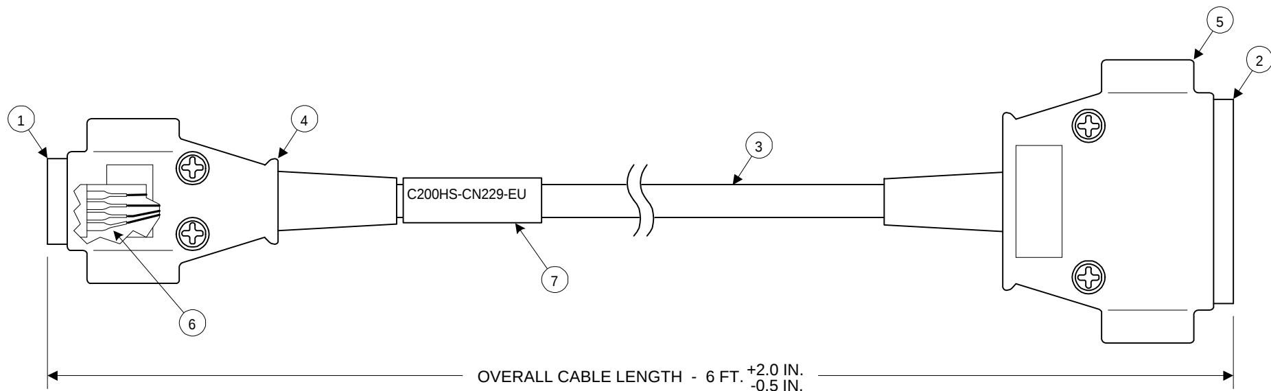
CABLE C200HS-CN229-EU
