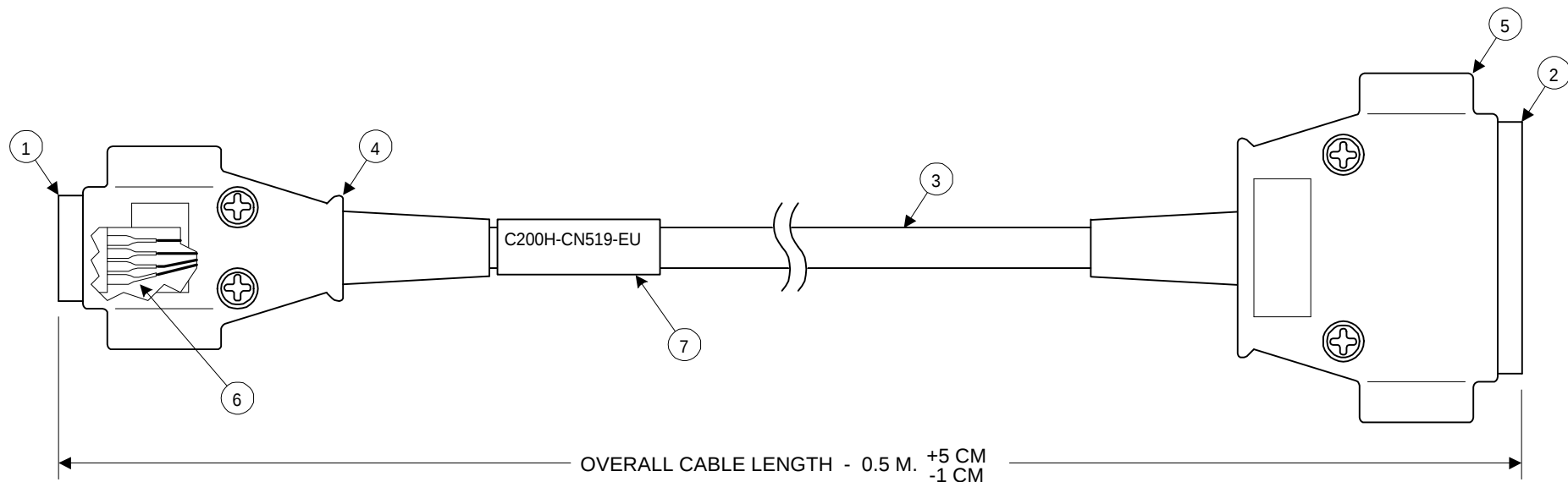
CABLE C200H-CN519-EU
