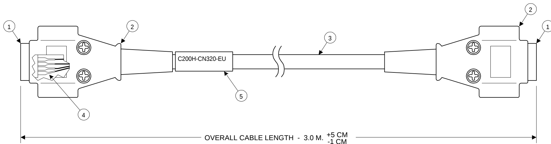
CABLE C200H-CN320-EU
