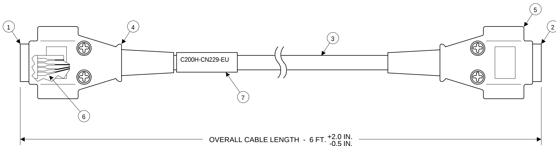
CABLE C200H-CN229-EU
