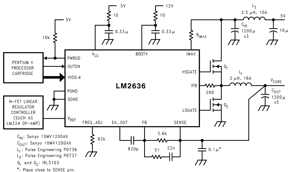
Figure 3. 5V to 1.3V–3.5V, 14A Power Supply
