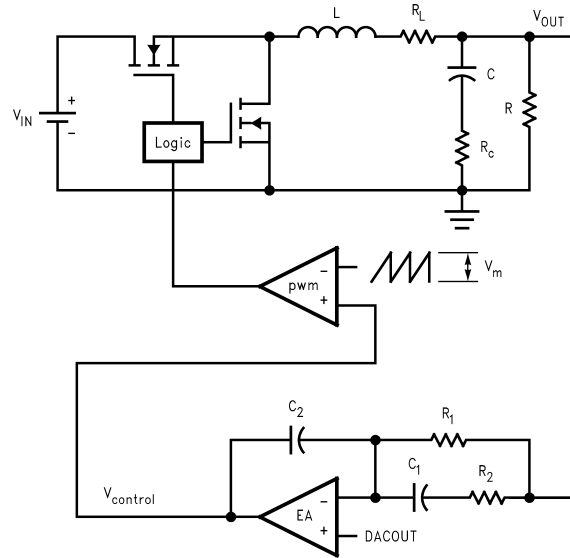
Figure 6. Buck Converter from a Control Point of View
