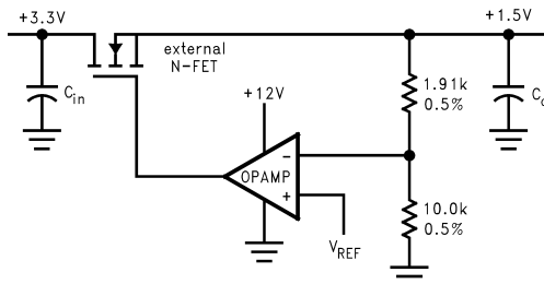
Figure 11. V_{REF} Used in an N-FET LDO Supply
