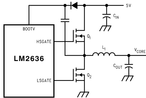
Figure 5. BOOTV Voltage Supplied by a Charge Pump
