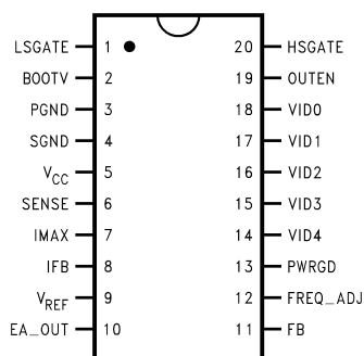
Figure 1. Plastic SOIC-20 (Top View) See Package Number DW
