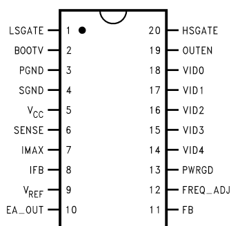
Figure 2. Plastic TSSOP-20 (Top View) See Package Number PW
