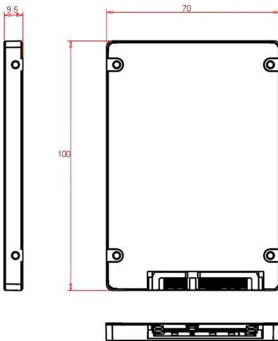
Figure 2: Physical Dimensions
