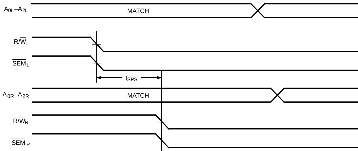
Figure 10. Timing Diagram of Semaphore Contention [38, 39, 40]
