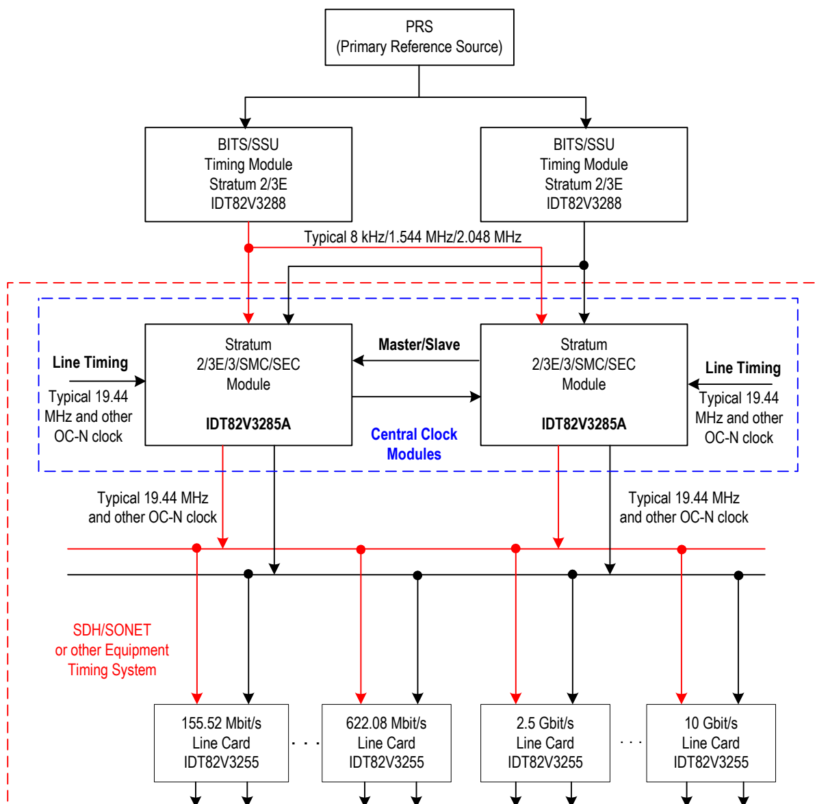
Figure 17. Typical Application
