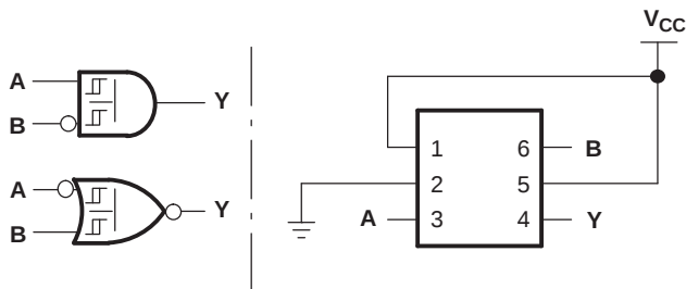
Figure 4. 2-Input AND Gate With Inverted B Input
