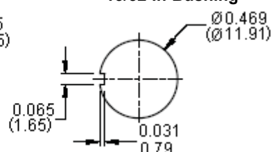
15/32 In Bushing
