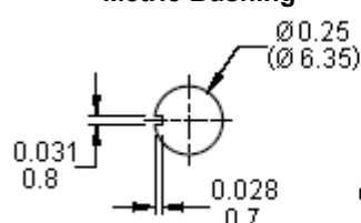
Metric Bushing
