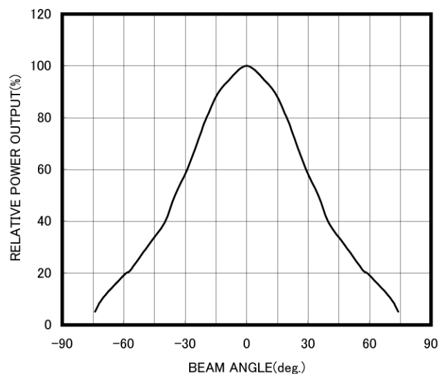
RADIATION PATTERN
