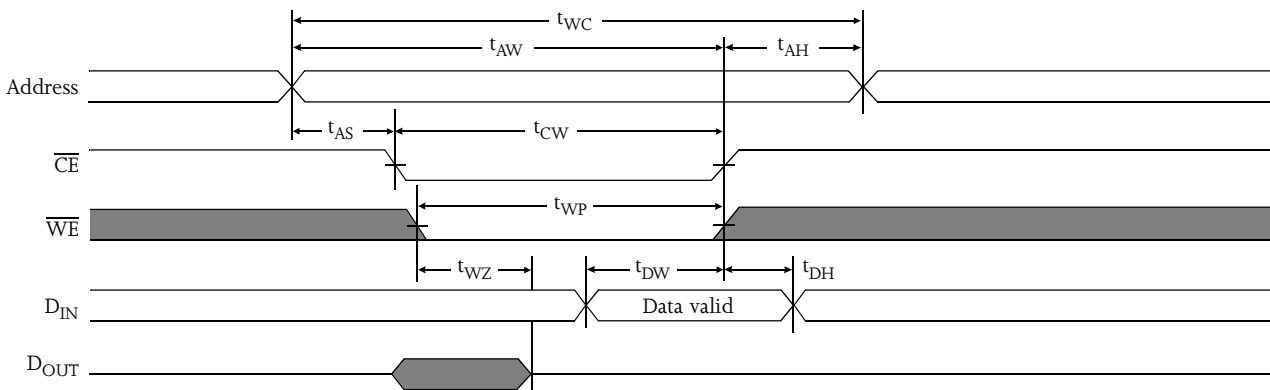
Write waveform 2 ( \overline{CE} controlled) 10,11
