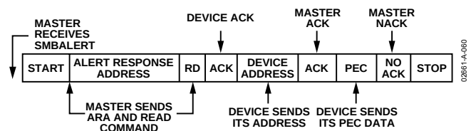
Figure 60. \overline{\text{INT/INT}} Responds to \overline{\text{SMBALERT}} ARA with Packet Error Checking (PEC)
