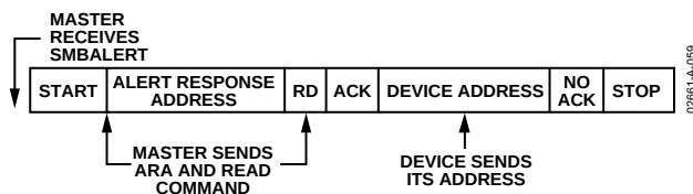
Figure 59. \overline{\text{INT/INT}} Responds to \overline{\text{SMBALERT}} ARA
