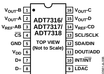
Figure 9. Pin Configuration QSOP
