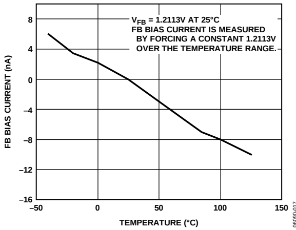
Figure 18. FB Bias Current vs. Temperature
