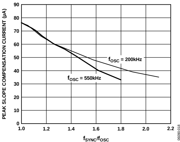
Figure 19. Slope-Compensation Current vs. f_{SYNC}/f_{OSC}
