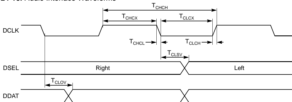
Figure 24-18. Audio Interface Waveforms
