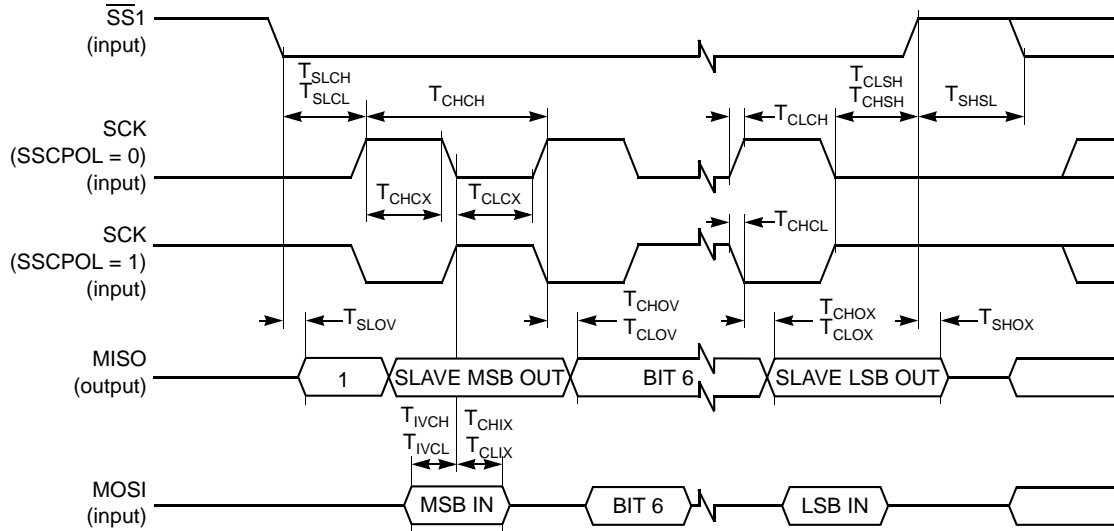
Figure 24-14. SPI Master Waveforms (SSCPHA = 0)
