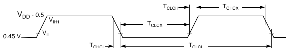
Figure 24-23. External Clock Waveform
