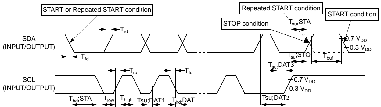
Figure 24-16. Two Wire Waveforms
