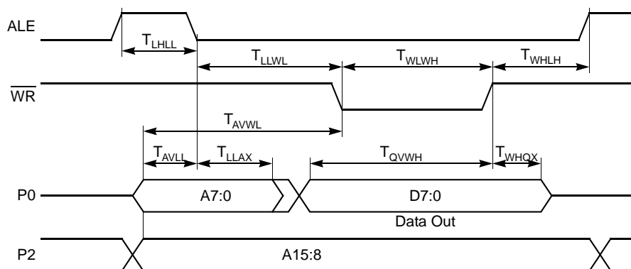
Figure 24-9. External 8-bit Bus Cycle – Data Write Waveforms
