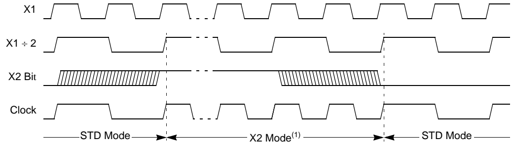
Figure 6-3. Mode Switching Waveforms
