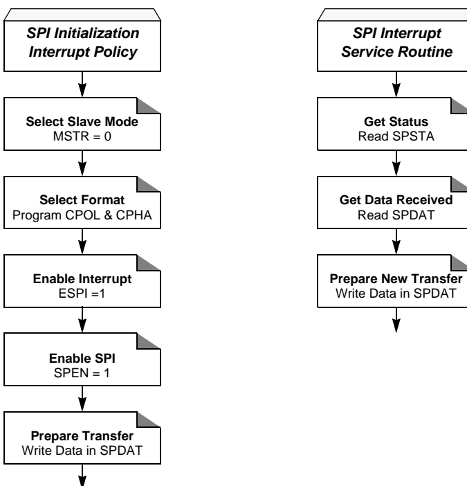
Figure 19-12. Slave SPI Interrupt Policy Flows
