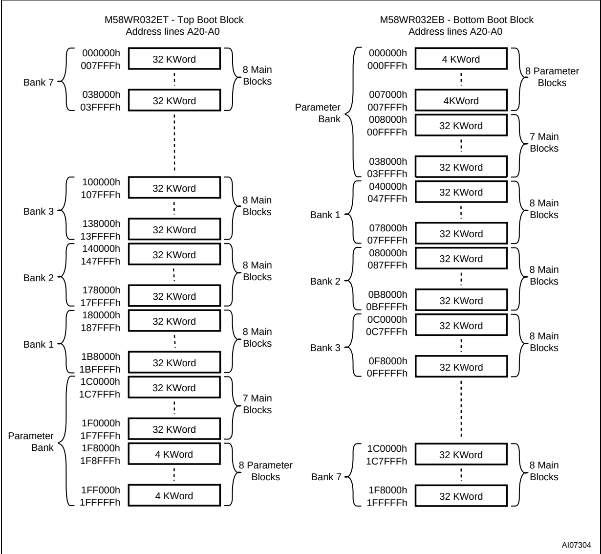
Figure 4. Memory Map
