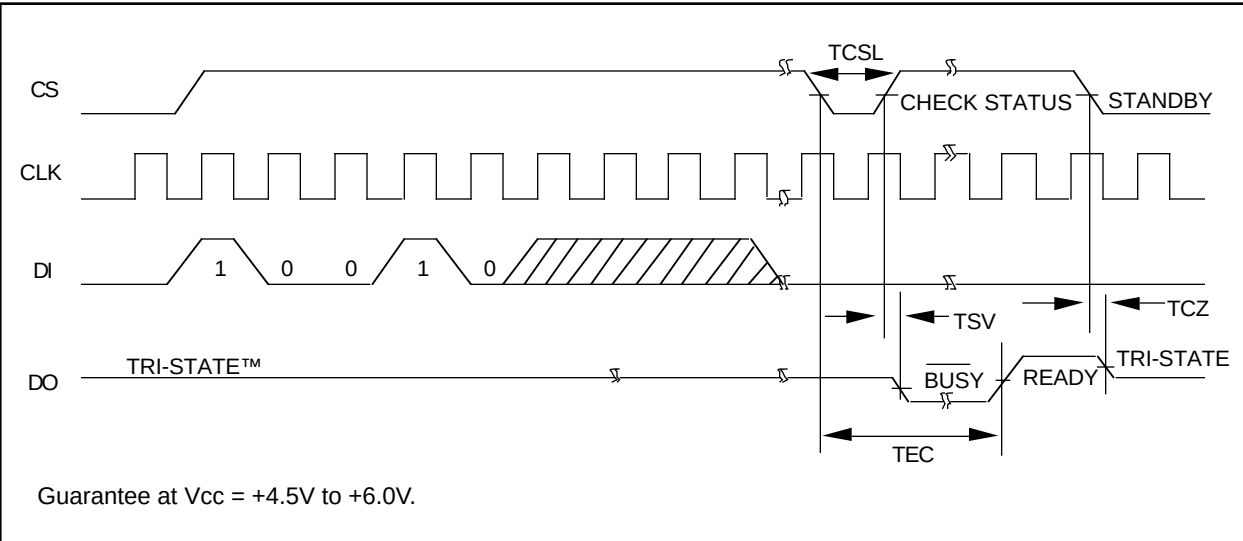
FIGURE 9-8: ERAL TIMING
