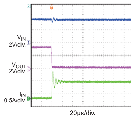
Short Output
