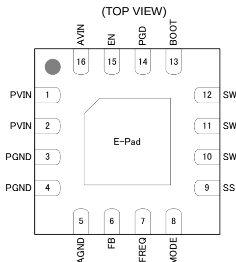
Figure 2. Pin Assignment
