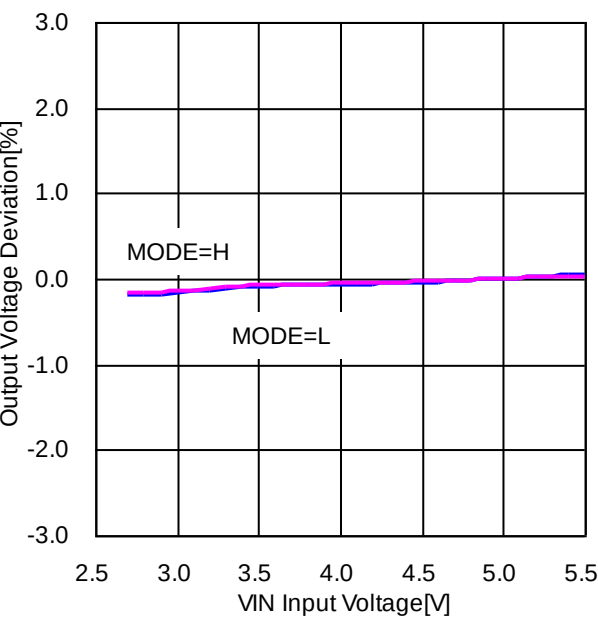
Figure 36. Line Regulation (VOUT=1.2V, L=1.0μH, FREQ=H, IOUT=5A)
