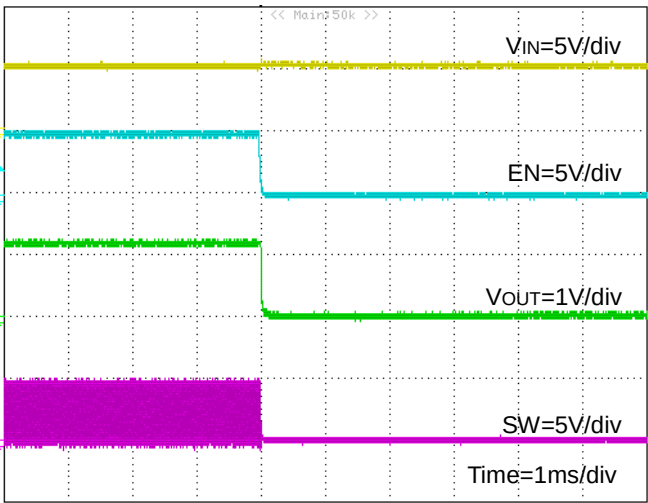
Figure 29. Power Down Waveform with EN (FREQ=H, RLOAD=0.24Ω)
