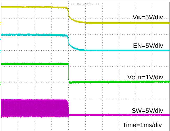
Figure 31. Power Down Waveform with VIN (FREQ=H, RLOAD=0.24Ω)
