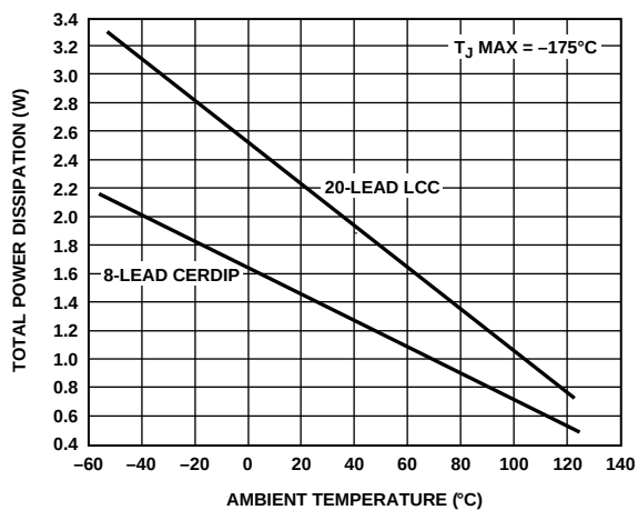
Figure 24. Maximum Power Dissipation vs. Temperature for Hermetic Packages
