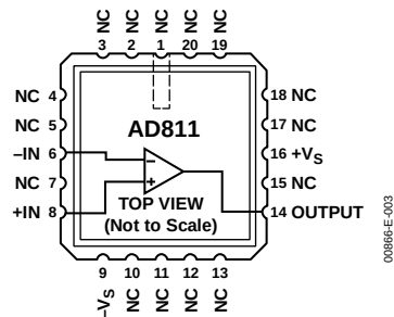
Figure 2. 16-Lead SOIC-W (RW-16)
