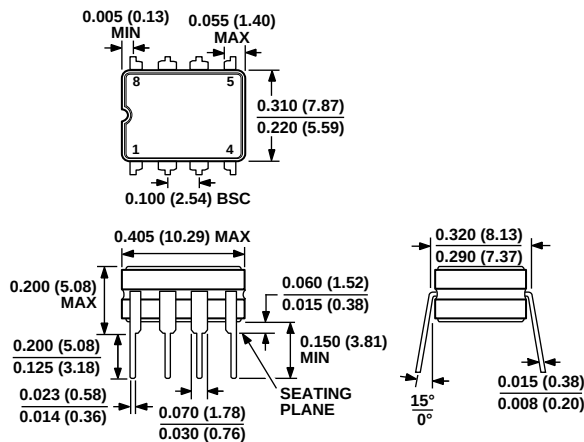
Figure 49. 8-Lead Plastic Dual In-Line Package [PDIP] (N-8)
