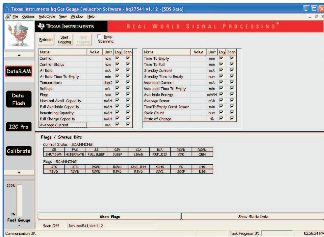
Figure 7. DataRAM Screen
