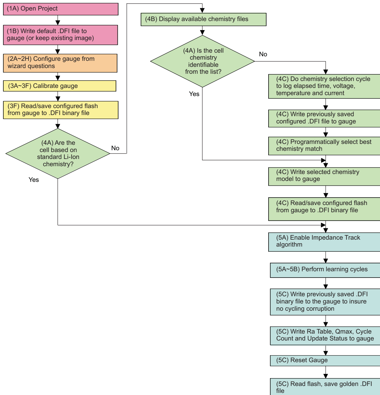
Figure 11. bqEasy™ Flowchart
