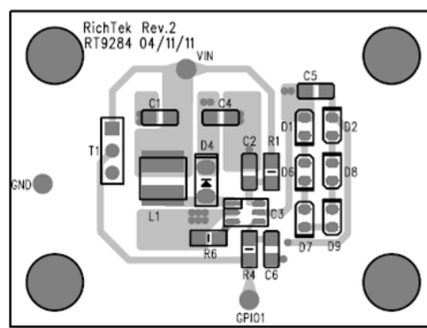
Figure 9. Top Layer
