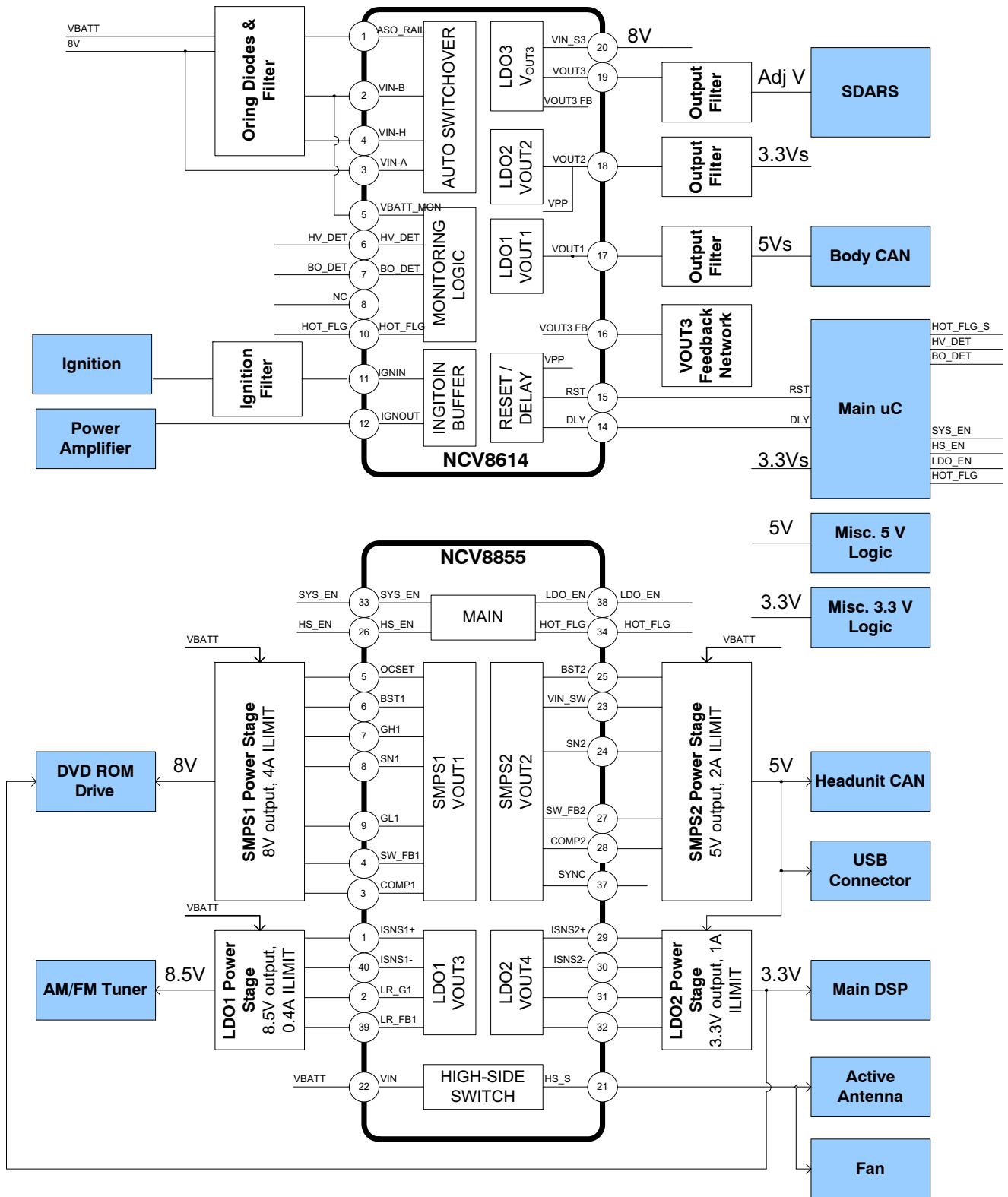
Figure 2. Automotive Radio System Block Diagram Example NCV8614 with NCV8855
