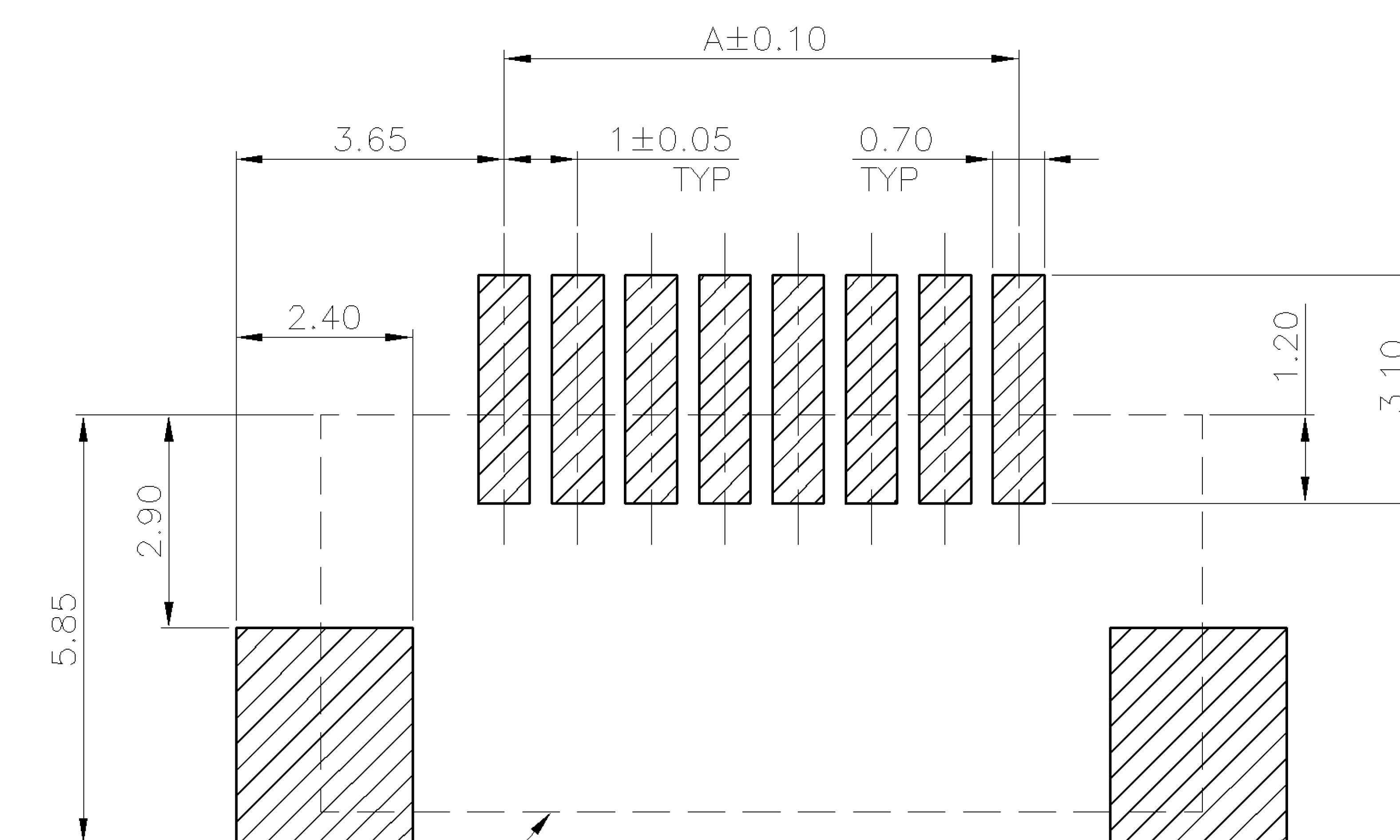
CONNECTOR OUTLINE
