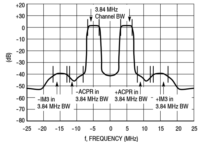
Figure 12. 2-Carrier W-CDMA Spectrum
