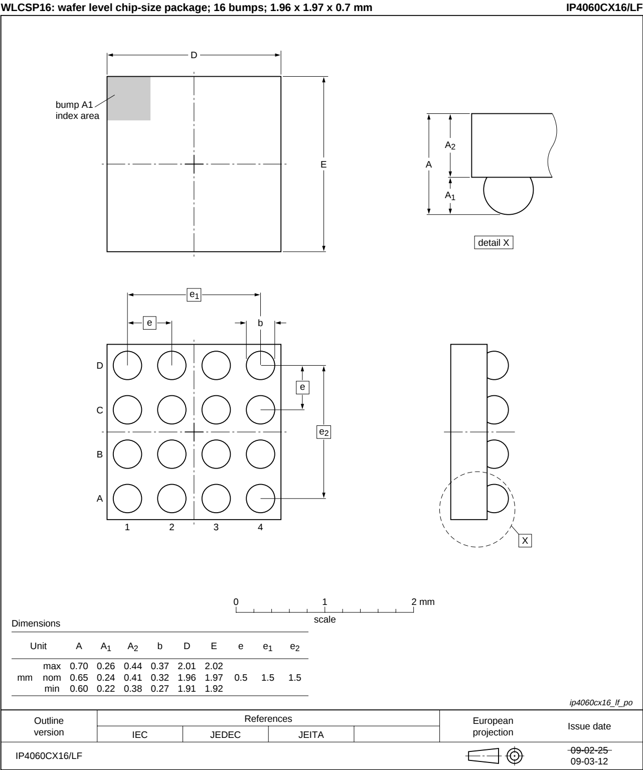
Fig 3. Package outline IP4060CX16/LF (WLCSP16)
