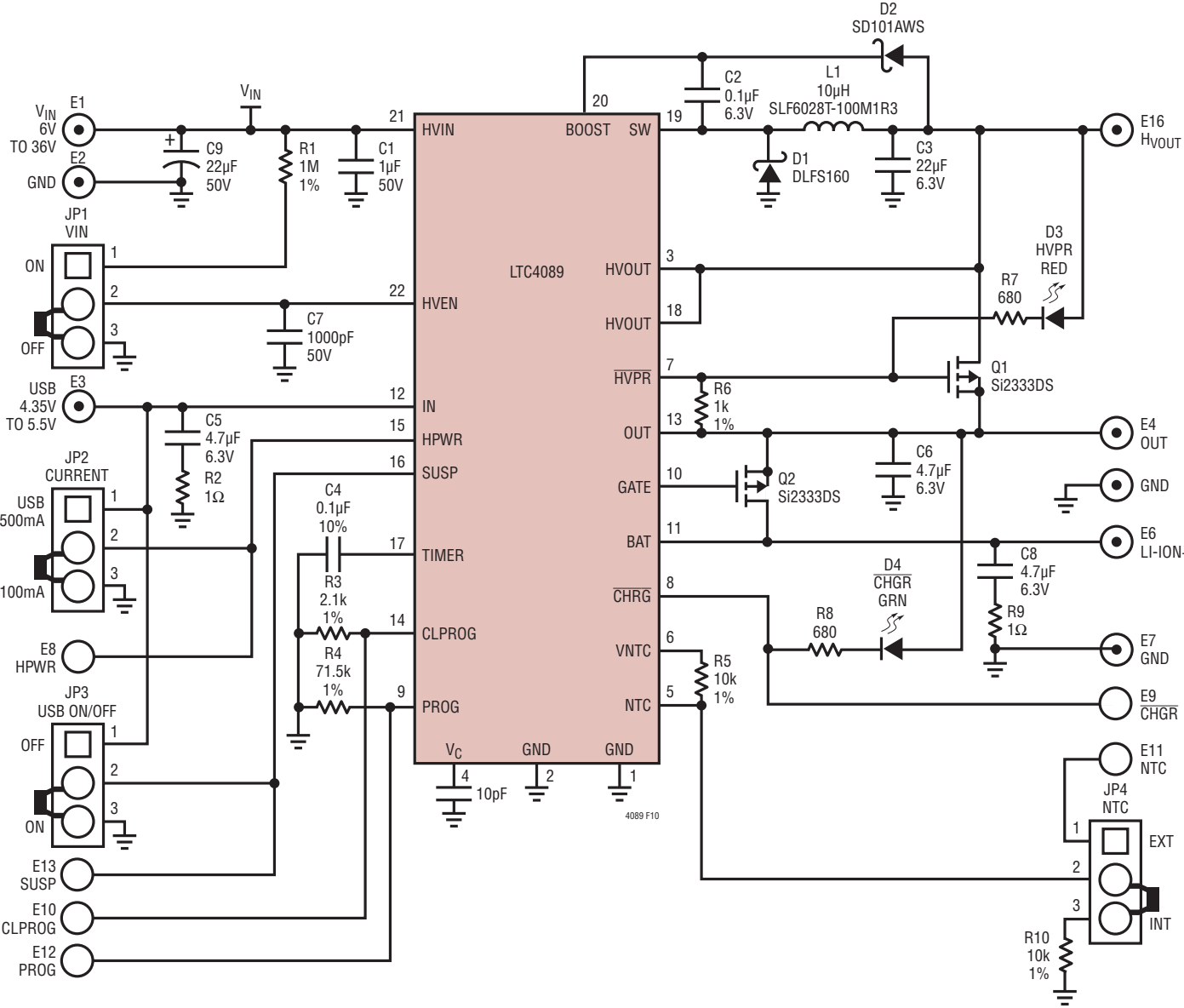
Figure 10. Typical Application Diagram
