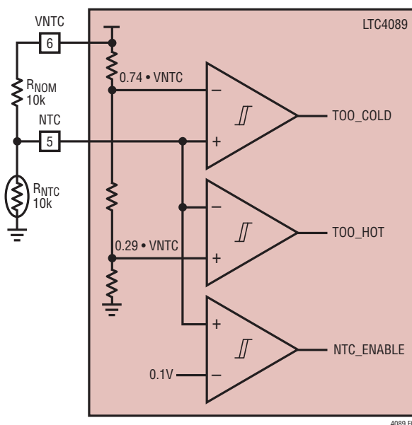
Figure 4. NTC Circuit
