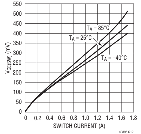
High Voltage Regulator Switch Voltage Drop
