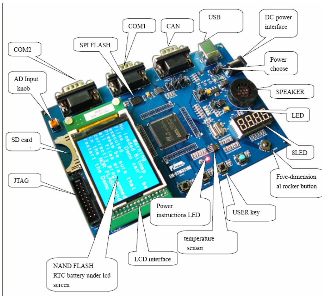
Figure 1.0 STM32F103ZE Board
