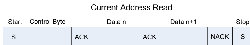
Figure 7.2 Current Address Read.
