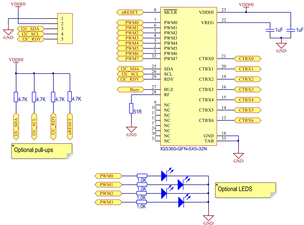
Figure 4.2 IQS360 Reference Design.
