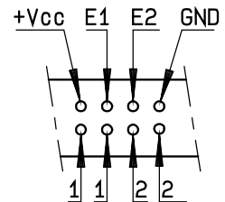
Solder pins
