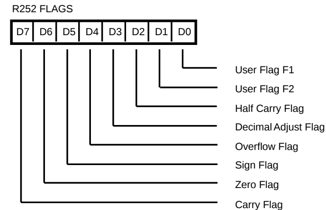
Figure 52. Flag Register FCH: Read/Write
