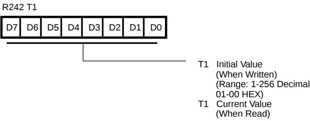
Figure 42. Counter/Timer 1 Register F2H: Read/Write
