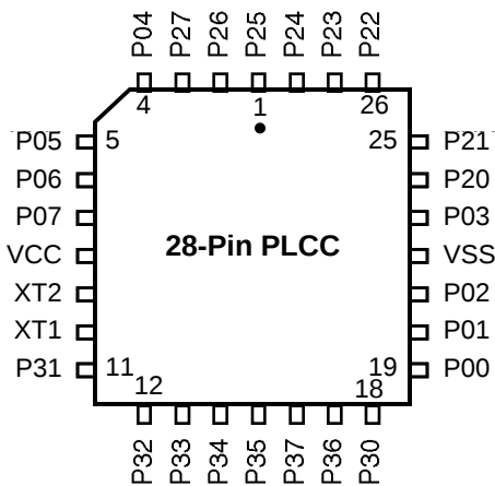
Figure 10. Standard Mode 28-Pin PLCC Pin Configuration
