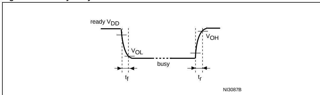
Figure 43. Ready/Busy AC waveform
