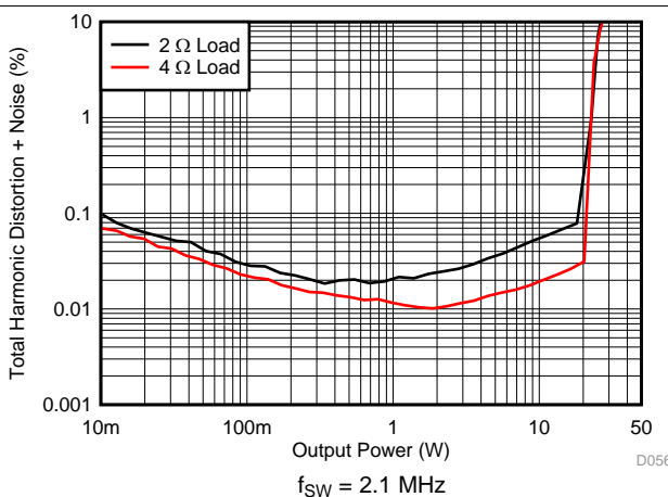
Figure 6. THD+N vs Power
