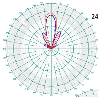
900-928 MHz H Plane
